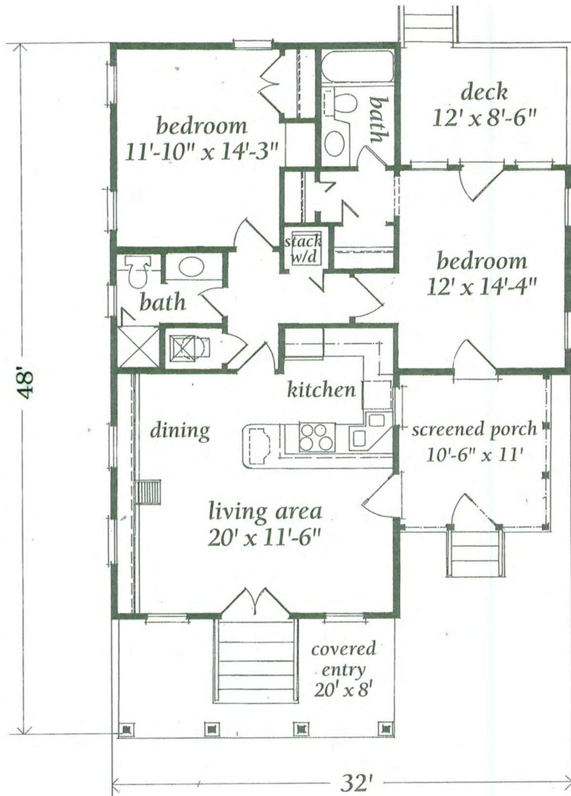
FIRST FLOOR (972 SQ. FT.)
