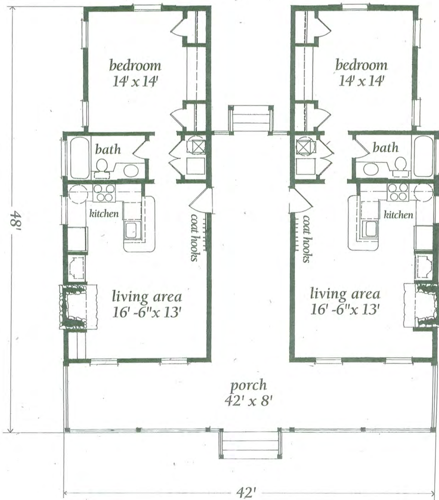
MAIN FLOOR (1,256 SQ. FT.)
